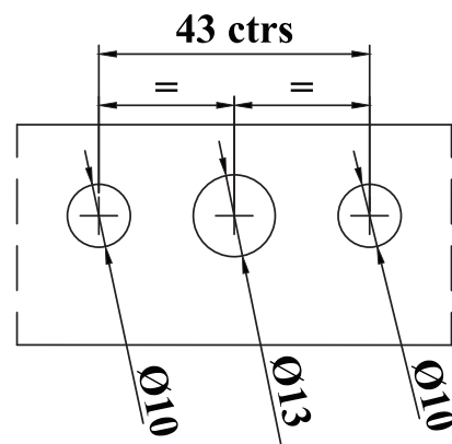
Figure 2: Holes for Handle Fitment
