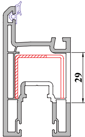
Figure 1: Super Sash Routing for Handle and Espagnolette Fitment
