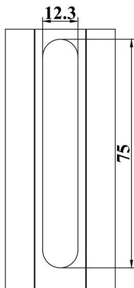
Figure 3: Routing for Espagnolette Gear Box Fitment
