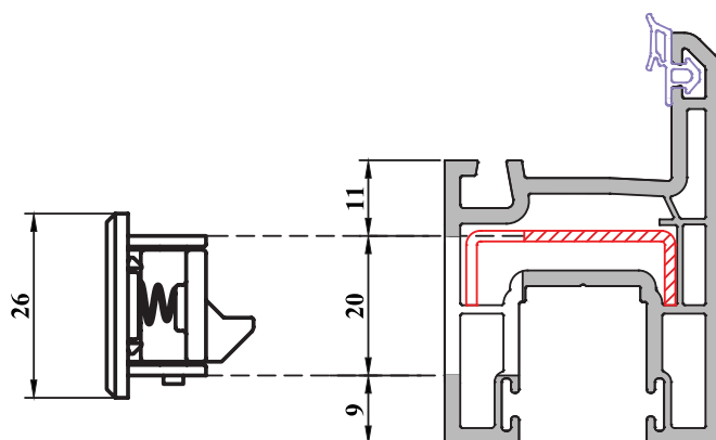
Sash routing for touch lock fitting
