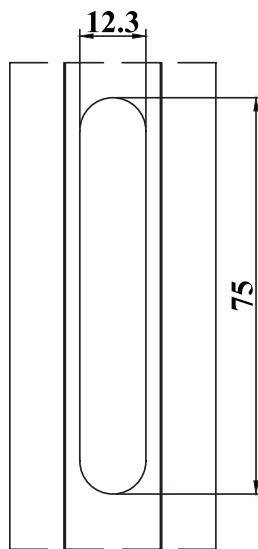
Figure 2: Routing for Espagnolette Gear Box Fitment
