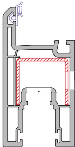
Figure 1: Sash Routing
