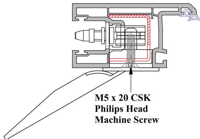
Figure 3: Assembly of Pop-up Handle
