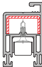
Super Screen Sash Profile 41321 - 03000
