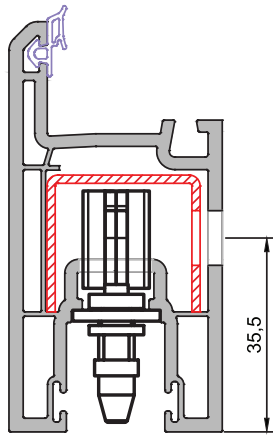
Figure 1: Sash Routing
