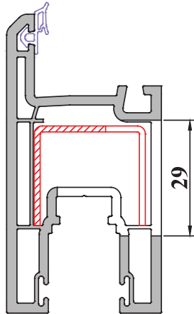
Figure 1: Super Sash Routing for Handle and Espagnolette Fitment
