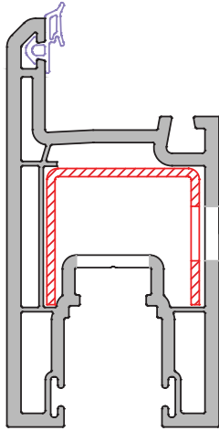
Figure 1: Sash Routing
