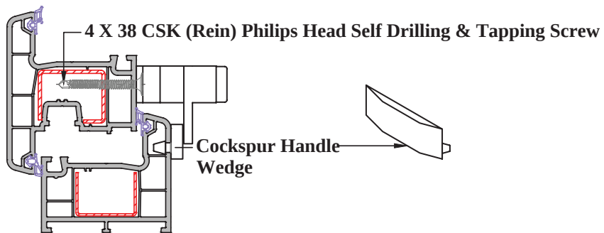
Holes for fixing Handle Wedge
