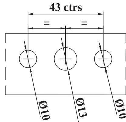
Figure 2: Holes for Handle Fitment
